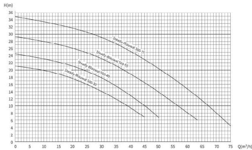
Steady-Blauwal 500-30/40
